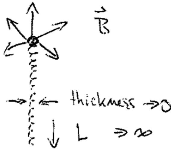
Figure 4.5: Magnetic monopole with Dirac string (infinitely long, infinitely thin solenoid) along the negative z -axis.
