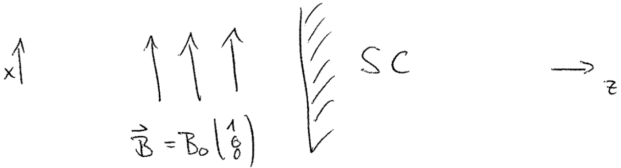
Figure 4.1: Magnetic field close to a superconductor exhibiting the Meissner effect.
