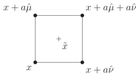
Figure 3.3: Plaquette associated with the site x , or \tilde{x} on the dual lattice.
