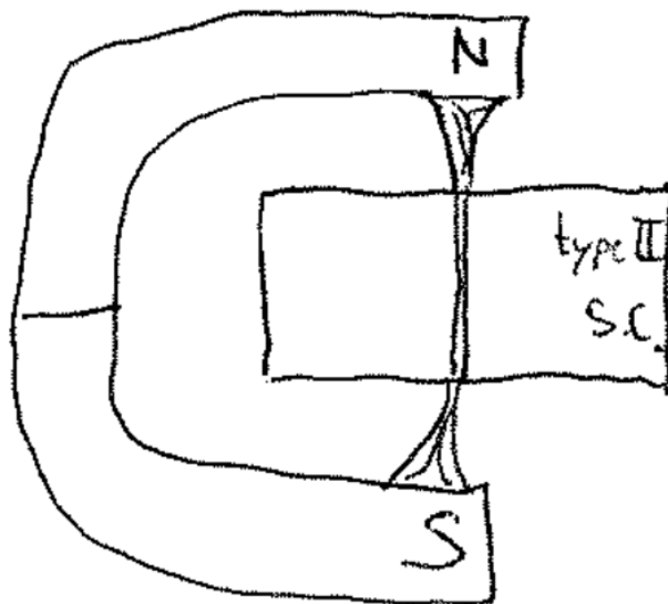
Figure 4.2: Abrikosov vortices penetrating a Type-II superconductor.
