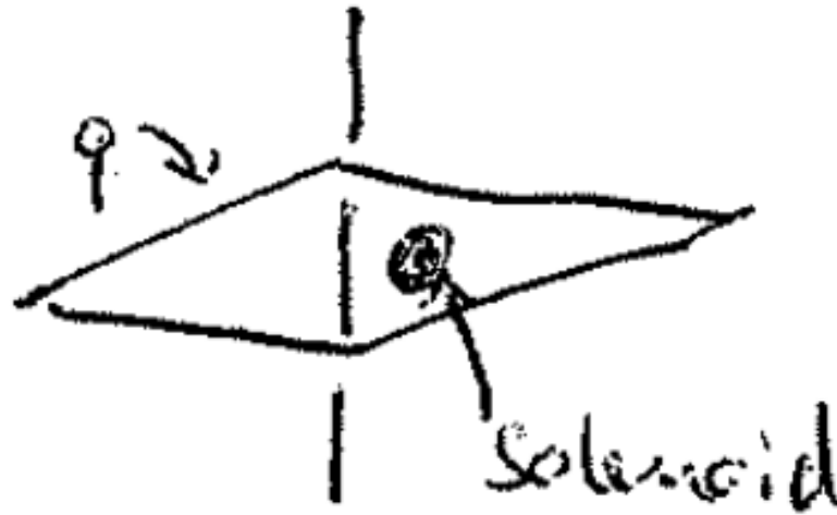
Figure 4.6: Aharonov-Bohm effect: Electron wavefunction split into two parts encircling a solenoid with magnetic flux \Phi . The interference pattern depends on \Phi even if the electrons never pass through a region with non-vanishing magnetic field.
