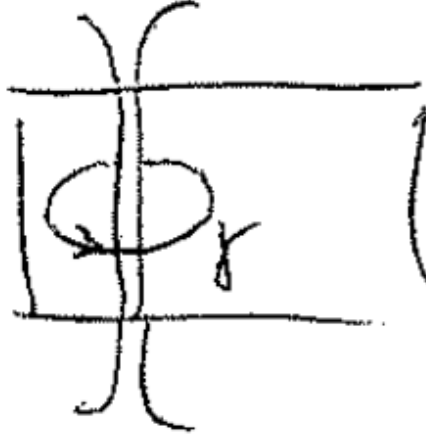
Figure 4.3: Contour \gamma around a magnetic vortex in a superconductor.
