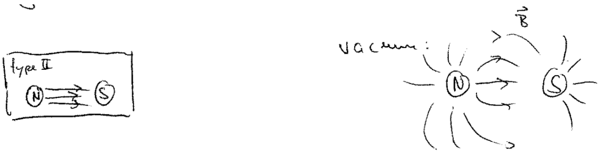
Figure 4.4: Magnetic flux string between two monopoles in a Type-II superconductor.
