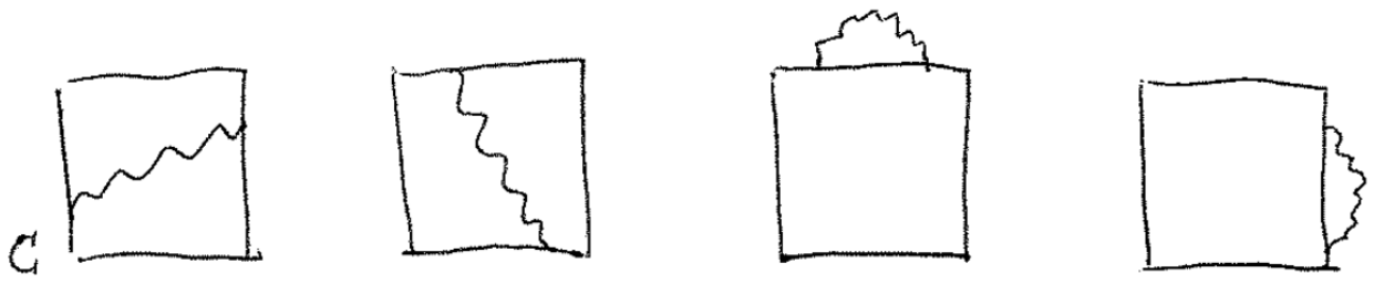
Figure 3.1: Different contributions to the exponent of the Wegner-Wilson loop expectation value in QED due to photon exchange between different segments of the rectangular contour \mathcal{C} .
