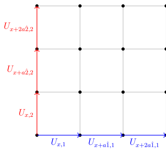
Figure 3.2: A 2D lattice with link variables U_{x\mu} \equiv U_{x,x+a\hat{\mu}} connecting neighboring sites.
