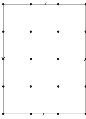
Figure 3.4: Rectangular lattice enclosed by a Wilson line (contour) \mathcal{C} .
